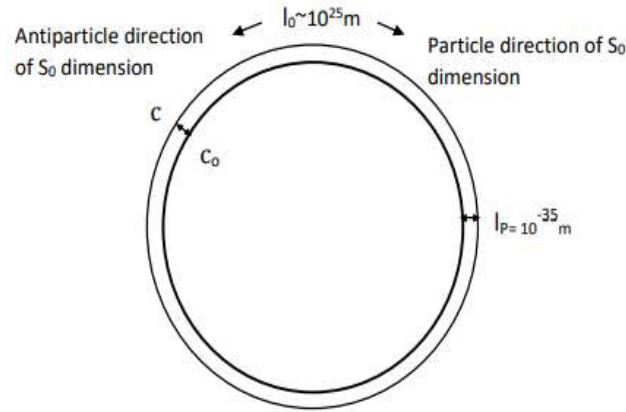
FIG. 3. Ring structure of S_0 - S_P dimensions with two unequal speed limit states C and C_o , at the two ends of S_P dimension.
