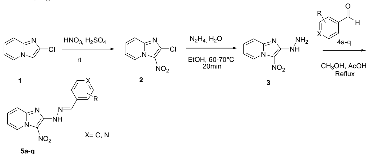
FIG.2. Synthesis route of compounds 5a-q
