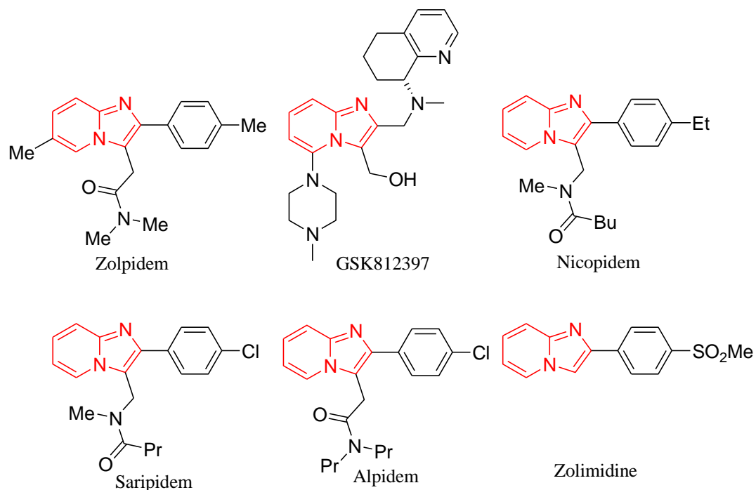
FIG.1. Imidazo[1,2-a]pyridine-containing drugs marketed.
