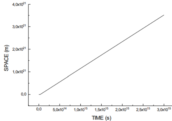
FIG. 1. Evolution of the universe.
