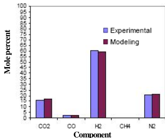
Figure 2: comparing the result of model with output data from TABLE 1 T_{out} of model= 410.364°C and T_{out} of experimental = 411°C
