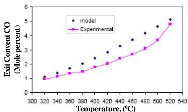
Figure 7: Comparing exit content CO in temperatures between 310-530°C from model with experimental data [12]
