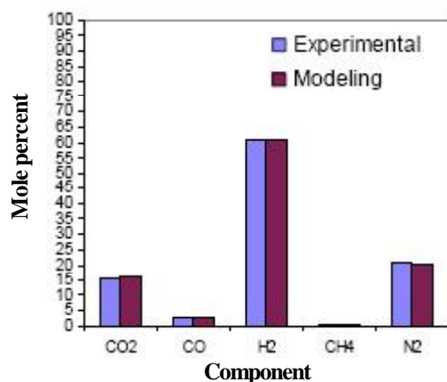
Figure 3: comparing the result of model with output data from TABLE 2 T_{out} of model= 411.305°C and T_{out} of experimental = 411°C
