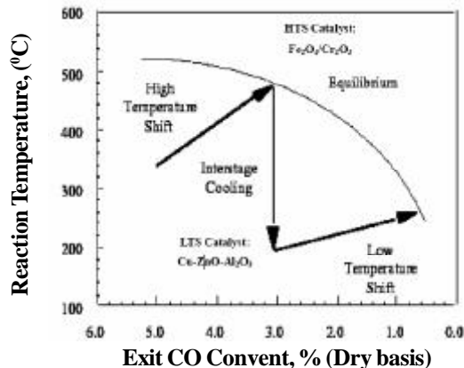
Figure 6: Schematic graph of water gas shift reaction [12]
