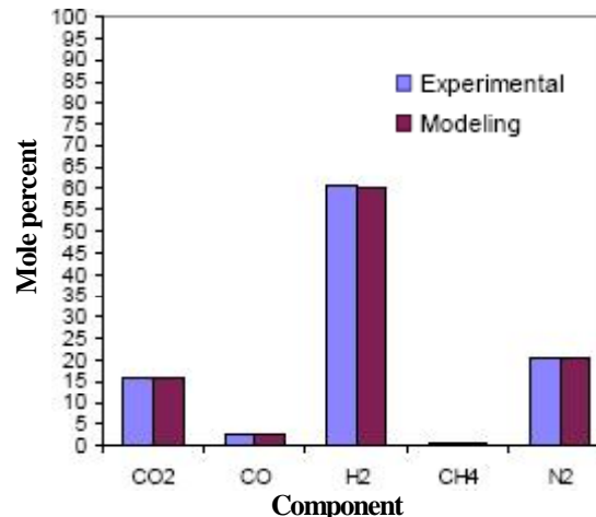
Figure 5: comparing result of model with output data from TABLE 4 T_{out} of model= 409.658°C and T_{out} of experimental = 412°C
