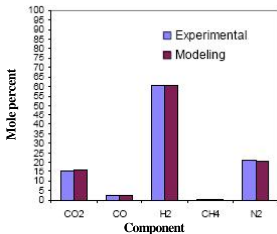
Figure 4: comparing the result of model with output data from TABLE 3 T_{out} of model= 411.067°C and T_{out} of experimental = 413°C
