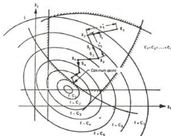
Figure 1: The optimization path for reformer reactor using the DFP optimization procedure
