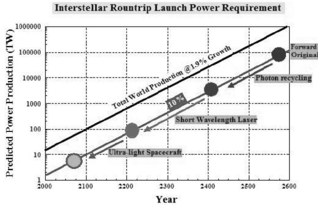
Figure 5 : A projection of the required power for PLT-BLP as a function of year based on the world power production projection by millis [8] .
