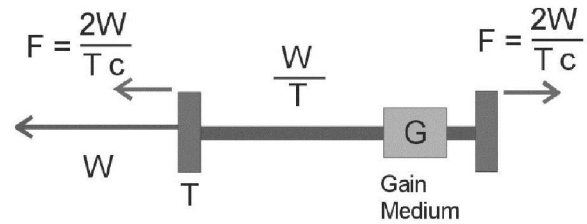
Figure 3 : Schematic diagram of the photonic laser thruster (PLT), which is based on the active resonant optical cavity approach to photon thrust amplification.
