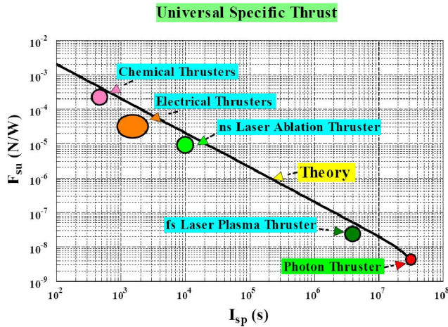
Figure 1 : The overall specific thrust (thrust to power ratio) of representative propulsion systems. Without photon thrust amplification, the specific thrust of photon thrusters follows the classic trend: the higher I_{sp} , the lower the specific thrust. The trend can be explained by the universal specific thrust in Eq. 12. However, with photon thrust amplification by recycling greater than 1,000, the photon thruster can be comparable with other conventional thrusters.
