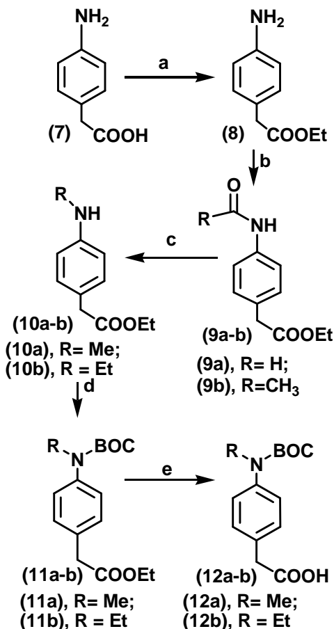
Scheme 2 : Reagents and conditions: a) EtOH, \text{H}_2\text{SO}_4 , reflux, 20 minutes; b) THF, (\text{RCO})_2\text{O} , -10 °C, 30 minutes; c) THF, \text{BH}_3 , DMS, RT, 1 hour; d) THF, di-tert-butyl dicarbonate, DMAP, reflux, 16 hours; e) MeOH, 1M LiOH, 50 °C, 30 minutes.
