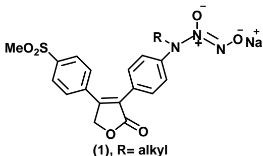
Figure 1 : Structure of putative hybrid nitric oxide donor N -diazen-1-ium-1,2-diolate derivatives of selective COX-2 inhibitory 4-[4-(methanesulphonyl)phenyl]-3-[4-(N-alkylamino)phenyl]-5H-furan-2-ones.
