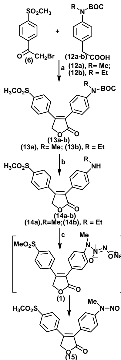
Scheme 3 : Reagents and conditions: a) 1. MeCN, \text{Et}_3\text{N} , 25 °C, 1 hour, 2. MeCN, DBU, 25 °C, 2 hours; b) MeOH, HCl, 25 °C, 1 hour; c) For 14a, Nitric oxide (40 psi), MeOH, ether, MeONa, 25 °C, 24 hours.
