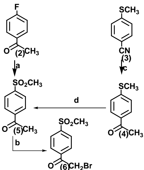
Scheme 1 : Reagents and conditions: a) DMSO, \text{CH}_3\text{SO}_2\text{Na} , 120 °C, 15 hours; b) \text{CHCl}_3 , \text{AlCl}_3 , \text{Br}_2 , -5 °C, 1 hour; c) 1. THF, MeLi, -78 °C, 2. 25 °C, 3 hours; 3. 3N HCl, 25 °C, 18 hours; d) \text{CH}_2\text{Cl}_2 , mCBPA, 18 hours.
