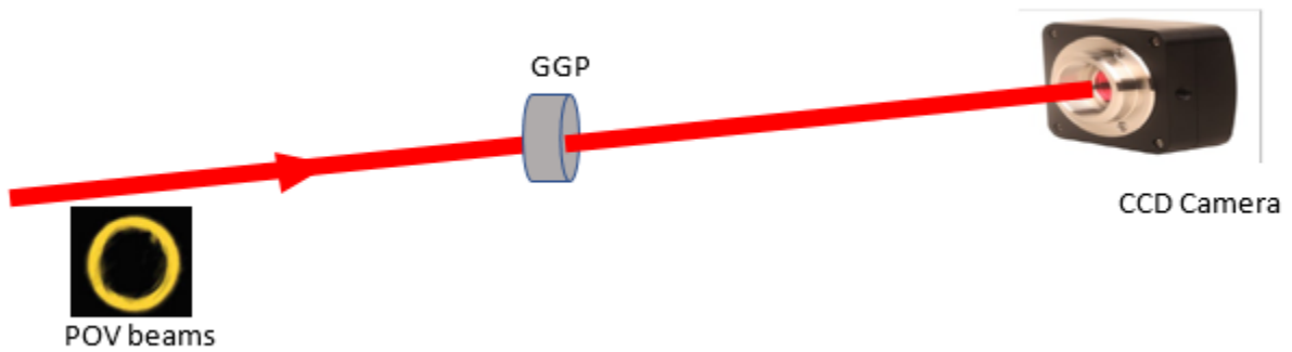
FIG. 2. Experimental set up for generation of speckle from POV beams using ground glass plate and recording the speckle pattern using CCD camera (color line).
