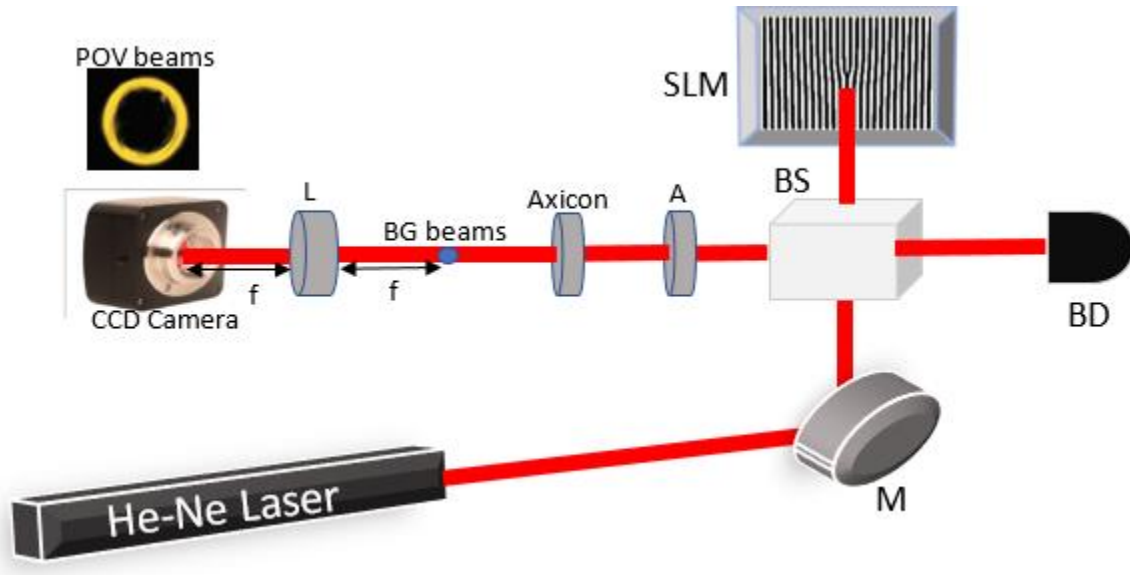
FIG. 1. Experimental setup for the generation of Perfect Optical Vortex (POV) beams using a spatial light modulator (in phase only mode) and an axicon (color line). M-Mirror, BD-Beam Dumper, BS-Beam Splitter, SLM-Spatial Light Modulator, A-Aperture, BG-Bessel Gauge, L-Lens, f-Focal Length, CCD-Charge Couple Device.
