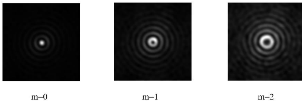
FIG.4. Represents experimentally generated Bessel-Gauss coherence functions of order m=0-2 at a propagation distance of 20 cm from the ground glass plate.
