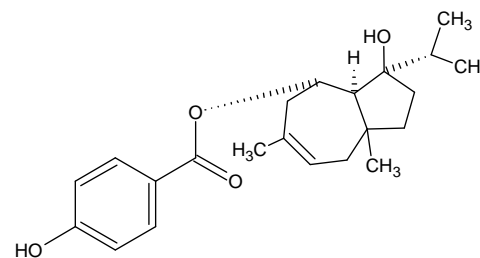
Ferutinine
