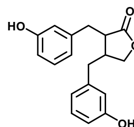
Enterolactone
