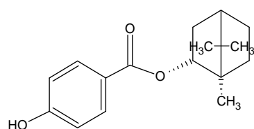
Tschimgine
