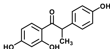
O-Desmethyl-angiolensin (O-DMA)
