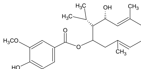
Tschimganidine
