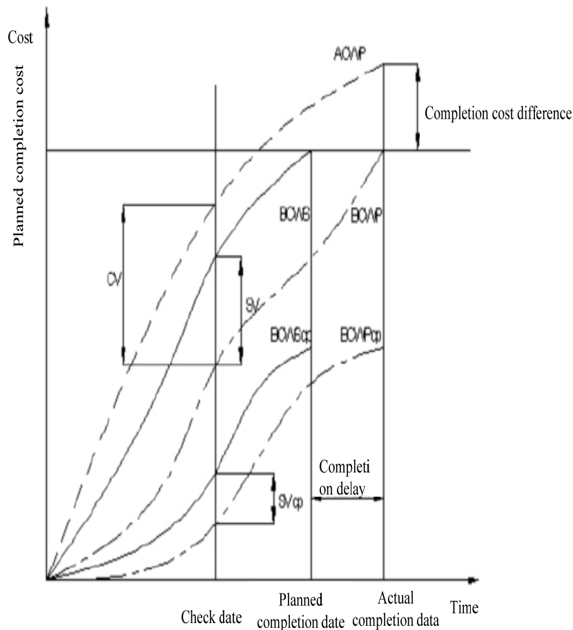
Figure 1 : Curve graph for evaluation of earned value method with critical paths
