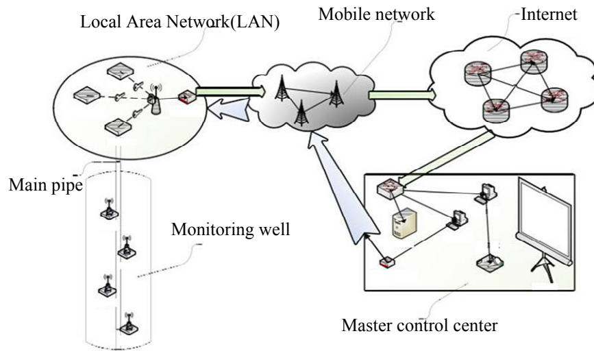
Figure 2 : Shallow ground temperature monitoring network
