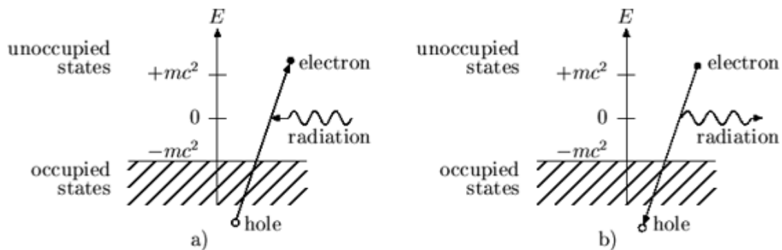
FIG.1. Dirac Hole Theory - Image Wikipedia a) electron/positron pair production b) annihilation.
