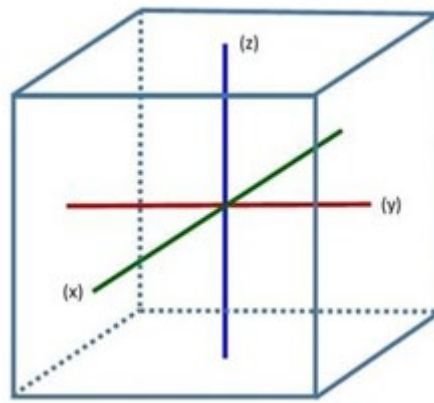
FIG 3.4 - Colour charge Cube
