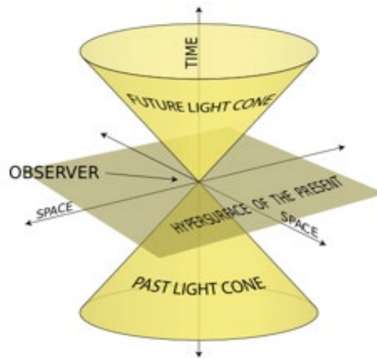
FIG. 5.2 - Light cone - Image Wikipedia
