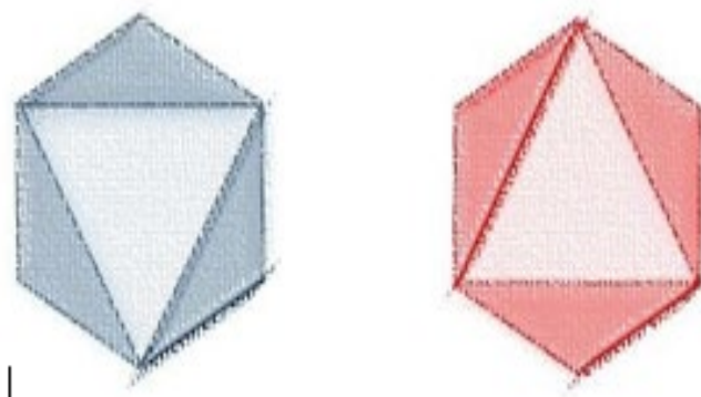
FIG.2.4. The Quark and the Antiquark
