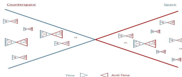
FIG. A.1 – Zero-point Matrix
