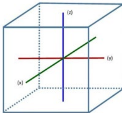
FIG. 2.6 - Cube - The three dimensions
