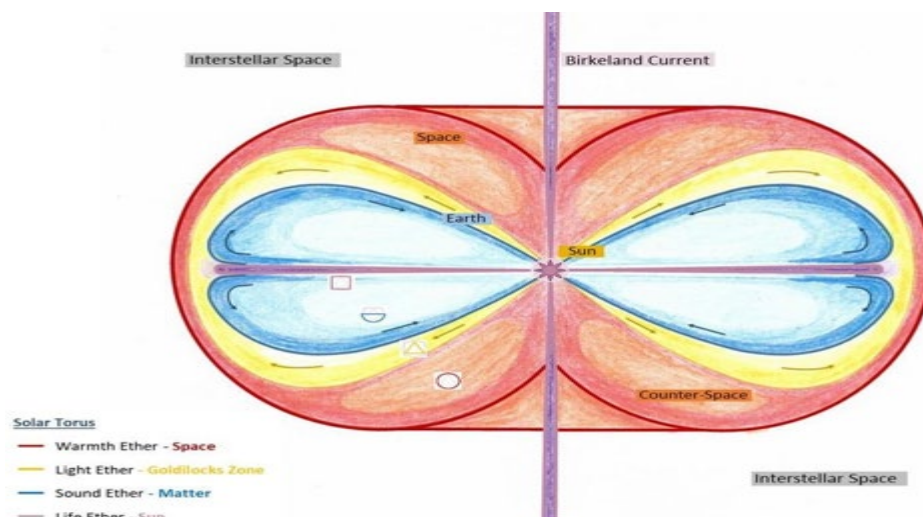
FIG. B.2 – Solar Torus Energy Fields
