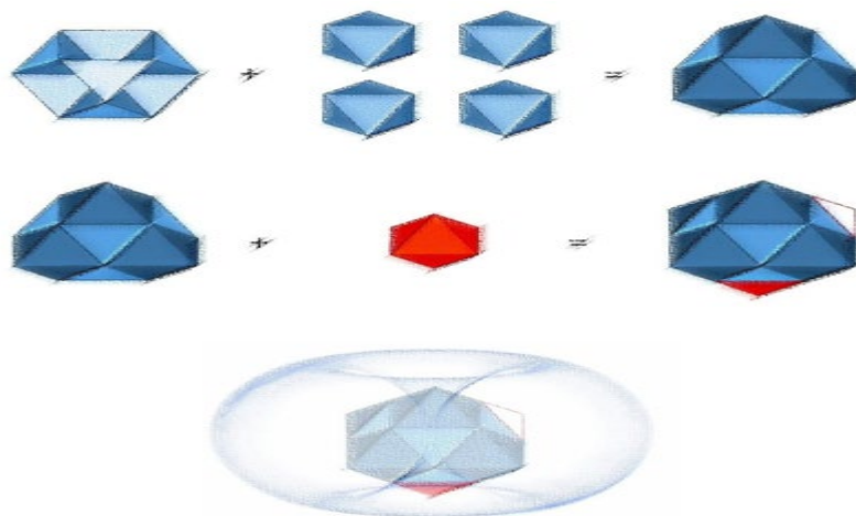
FIG. 3.3 - The Proton (+1)
