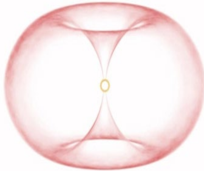
FIG. 5.1 - The sun torus (heliosphere)
