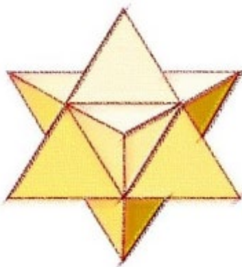
FIG. 2.8 - Star-tetrahedron
