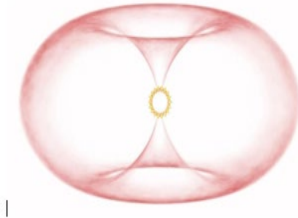
FIG.2.3. Solar torus - The Sun
