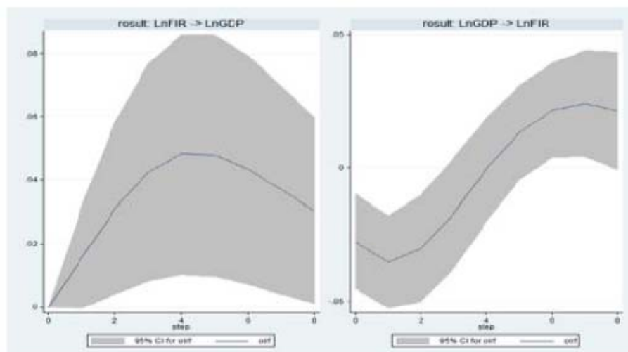
Figure 1: Impulse-response analysis
