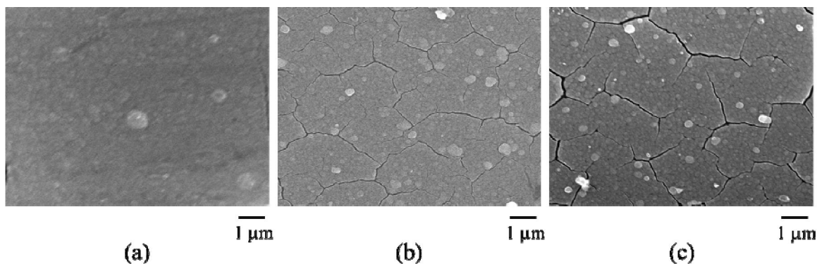
Figure 3 : Surface morphology of the titania films prepared by the normal LPD process, The raw solution temperatures are (a) 55 °C, (b) 60 °C, and (c) 65 °C, The \text{H}_3\text{BO}_3 solution concentration and deposition time are 0.3 mol/l and 5 hours, respectively
