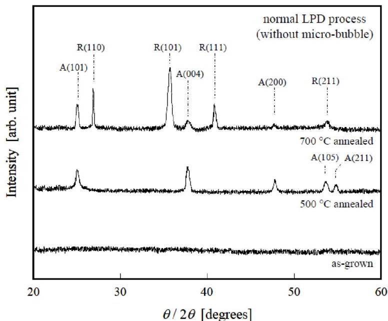
Figure 5 : XRD patterns of the titania film prepared by a normal LPD process (Figure 3 (b)) before and after annealing, A and R refer to the anatase and rutile planes, respectively
