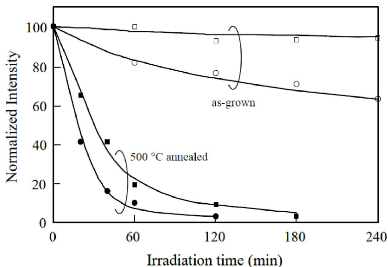
Figure 7 : Absorbance of methyleneblue at 654 nm as a function of UV light irradiation time, Squares represent the normal LPD films and circles represent the improved LPD films
