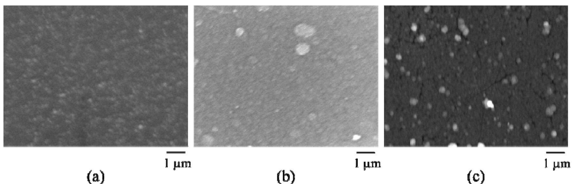
Figure 2 : Surface morphology of the titania films prepared by a normal LPD process, The H 3 BO 3 solution concentrations are (a) 0.1 mol/l, (b) 0.3 mol/l, and (c) 0.5 mol/l. The raw solution temperature and deposition time are 55 °C and 5 hours, respectively
