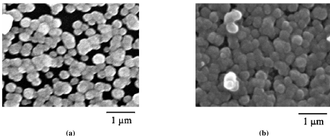
Figure 4 : Surface morphology of the titania films prepared by the improved LPD process, Deposition times are (a) 3 hours and (b) 5 hours, The \text{H}_3\text{BO}_3 solution concentration and the raw solution temperatures are 0.3 mol/l and 60 °C, respectively
