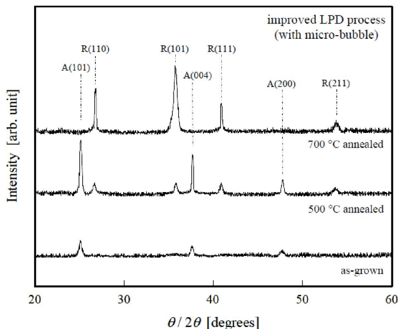
Figure 6 : XRD patterns of the titania film prepared by an improved LPD process (Figure 4) before and after annealing, A and R refer to the anatase and rutile planes, respectively
