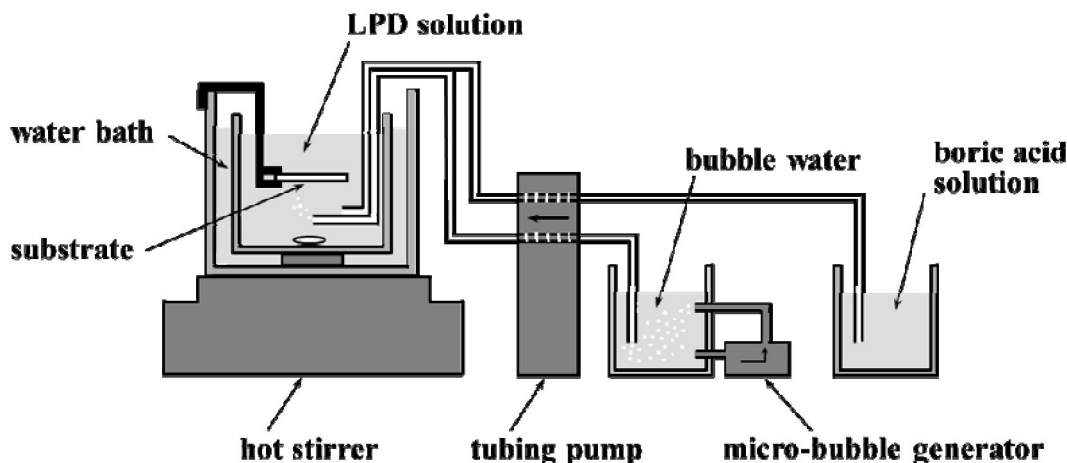
Figure 1 : A schematic diagram of the improved LPD system
