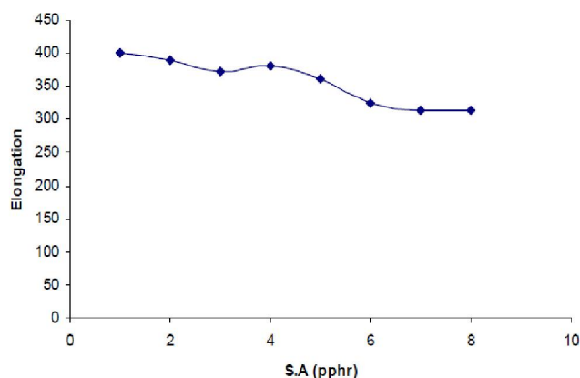
Figure 6 : Effect of (Saticric acid) on the SBR Elongation
