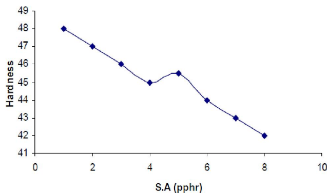
Figure 7 : Effect of (Satiric acid) on the SBR Hardness
