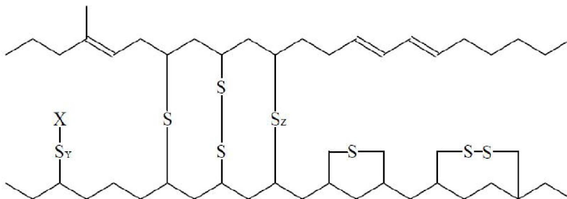
Figure 3 : Structural features of an accelerated sulfur vulcanizate of SBR Rubber (X= accelerator fragment).
