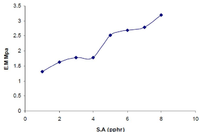
Figure 5 : Effect of (Saticric acid) on the SBR Elasticity
