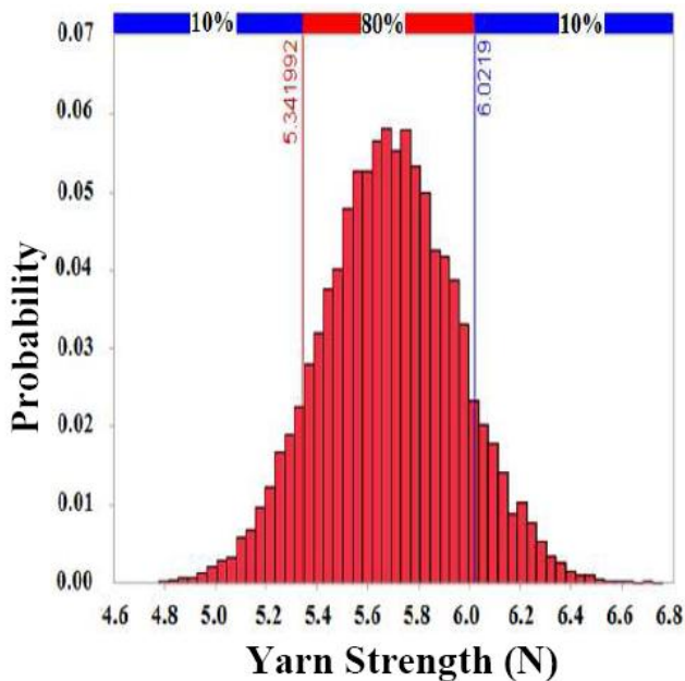
Figure 1 : Histogram plot
