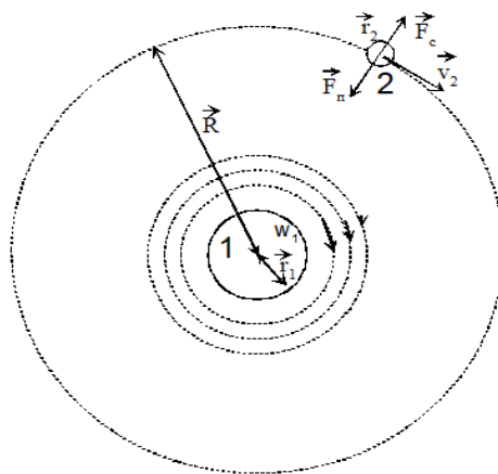
FIG.1. Two-dimensional model of gravitational interaction of two bodies.
