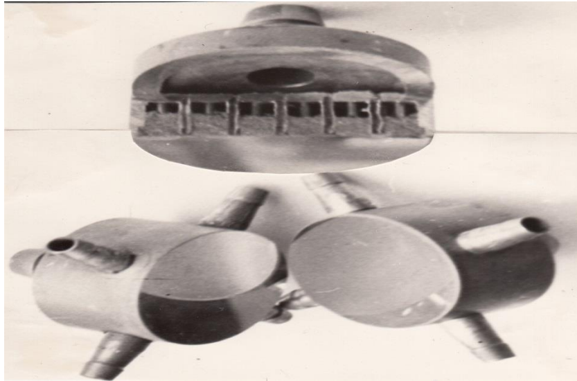
FIG. 2. First high power water cooled porous mirrors.
