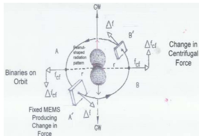
Figure 2 : Radiation pattern calculated by Landau and Lifshitz [4] (1975) Section 110 Page 356.
