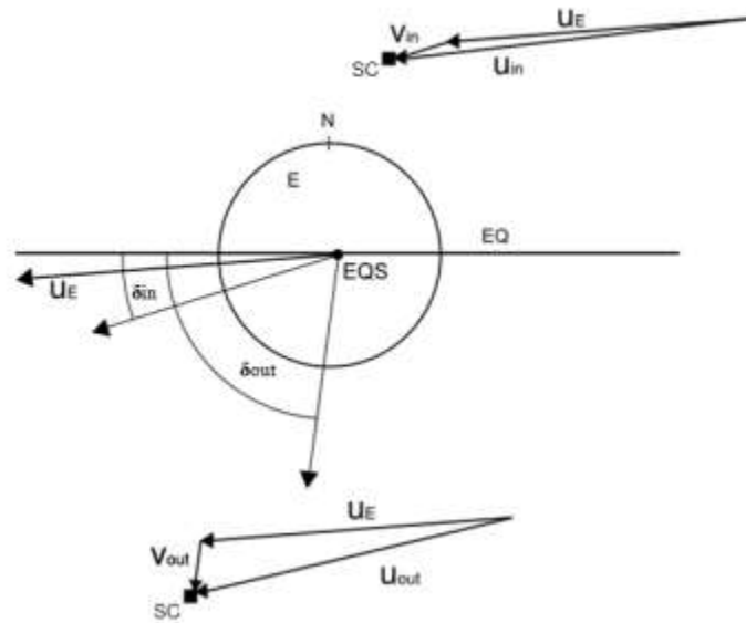
FIG. 1 Schematic visualization of the absolute velocity vector \vec{u}_e of Earth and the relative, asymptotic pre-encounter velocity vector \vec{v}_{in} , the relative, asymptotic post-encounter velocity vector \vec{v}_{out} of a Spacecraft (SC) in the Equatorial Frame (EQS), their declination angles \delta_{in} and \delta_{out} , and the derived absolute asymptotic pre-encounter and post-encounter velocity vectors \vec{u}_{in} and \vec{u}_{out} of a spacecraft during a gravity assisted flyby manoeuvre.
