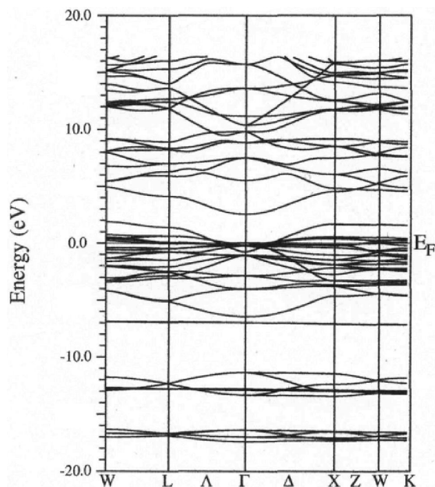
Figure 2 : The electronic band structure of \text{In}_2\text{MgTiO}_6 along high symmetry directions.
