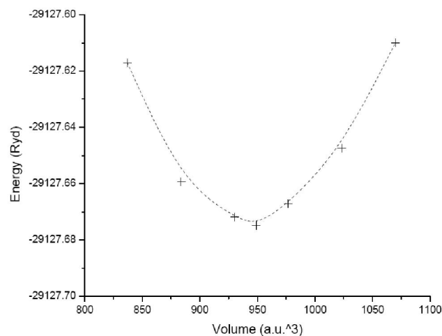
Figure 1 : Total energy of \text{In}_2\text{MgTiO}_6 as a function of cell volume.
