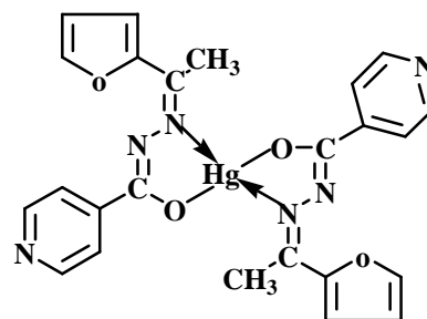
Figure 2 : Structure of Hg (II) complex with AFINH
