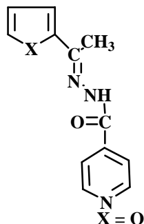
Figure 1 : Structure of AFINH
