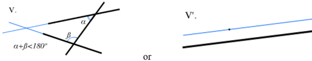
FIG. 2. Euclidean axiomatics.
