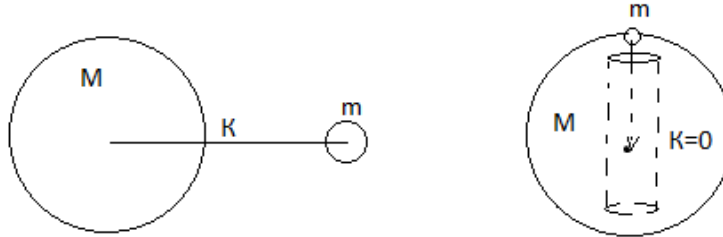
FIG. 6. Newton's law.
