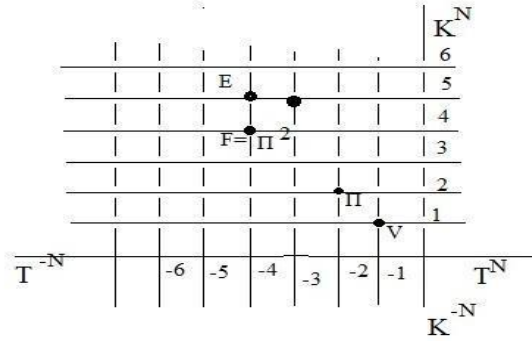
FIG. 5. Unified criteria for the evolution of space-matter.
