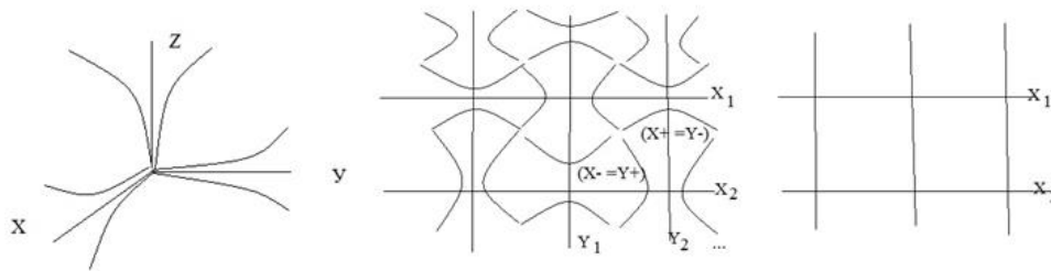
FIG. 3. Dynamic space-matter.
