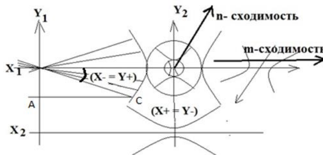
FIG. 4. Dynamic space-matter.
