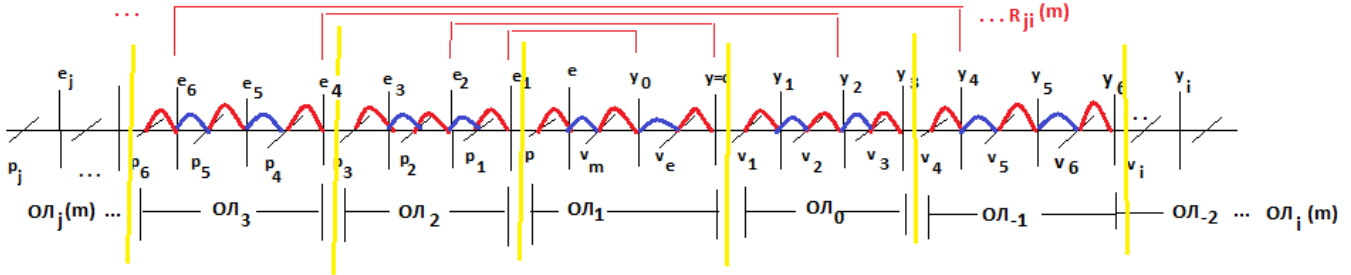
FIG. 7. Spectrum of indivisible quanta.
