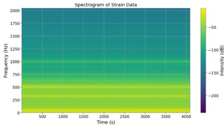
FIG. 11. Graph of spectrograms (strain data's frequency versus time).
