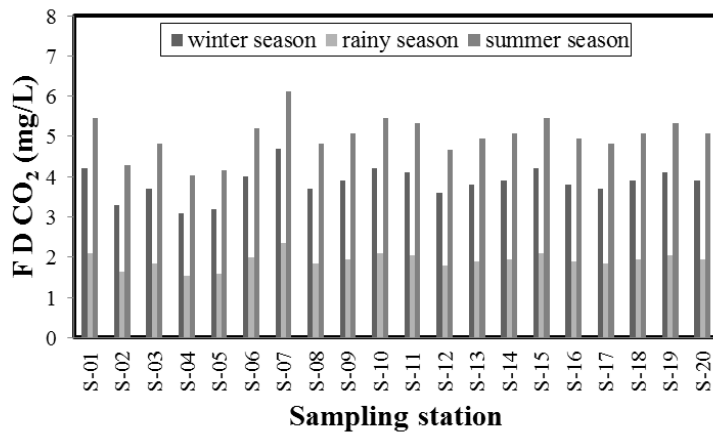
FIG. 10. Seasonal variations of Free Dissolved CO 2 of the Sundarbans Mangrove Forest river system in Bangladesh.
