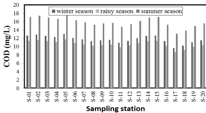
FIG. 13. Seasonal variations in concentration of Chemical Oxygen Demand (COD) of Sundarbans Mangrove Forest river system in Bangladesh.
