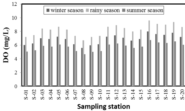
FIG. 11. Seasonal variations in concentration of Dissolved Oxygen (DO) of Sundarbans Mangrove Forest river system in Bangladesh.
