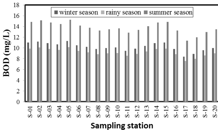
FIG. 12. Seasonal variations in concentration of Biological Oxygen Demand (BOD) of Sundarbans Mangrove Forest river system in Bangladesh.
