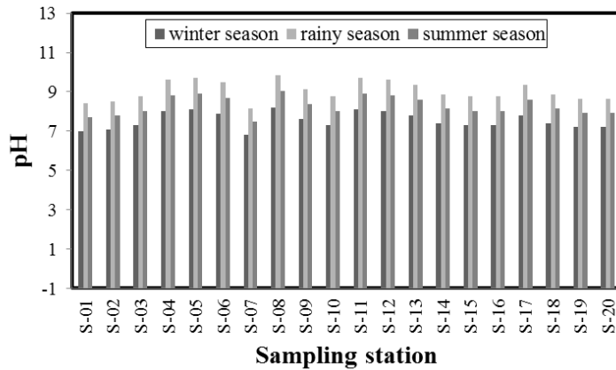
FIG. 3. Seasonal variations of pH of the Sundarbans Mangrove Forest river system in Bangladesh.
