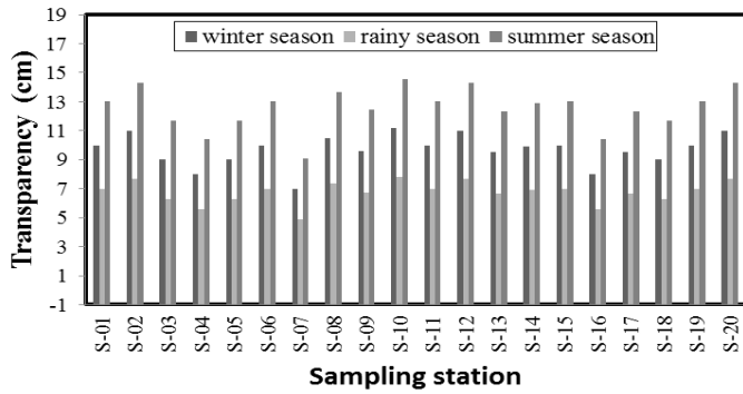
FIG. 5. Seasonal variations of Transparency of the Sundarbans Mangrove Forest river system in Bangladesh.
