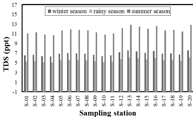
FIG. 6. Seasonal variations of TDS of the Sundarbans Mangrove Forest river system in Bangladesh.
