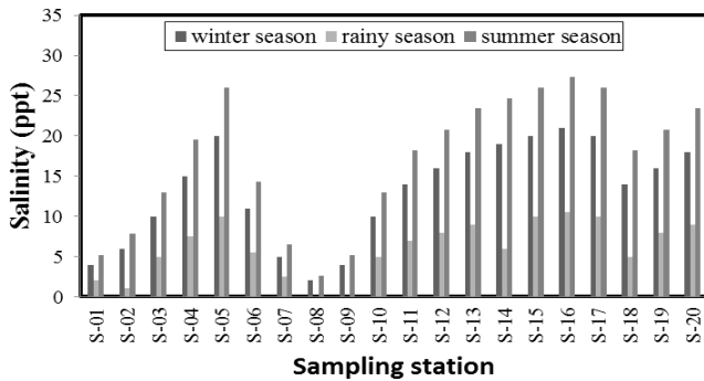
FIG. 7. Seasonal variations of Salinity of the Sundarbans Mangrove Forest river system in Bangladesh.
