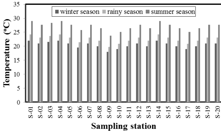
FIG. 2. Seasonal variations of temperature of the Sundarbans mangrove forest river system in Bangladesh.
