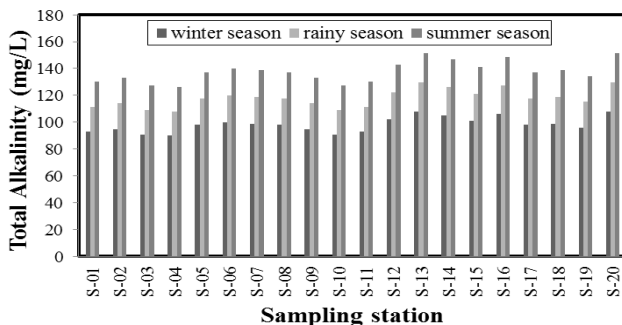
FIG. 8. Seasonal variations of Total Alkalinity of the Sundarbans Mangrove Forest river system in Bangladesh
