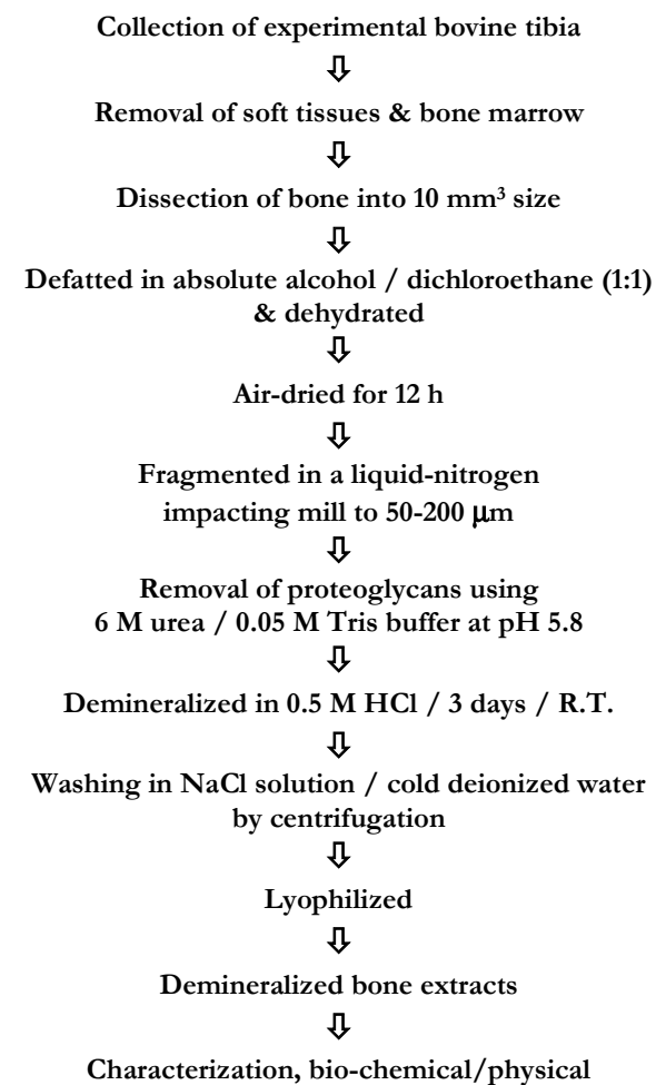
SCHEME 1: A representative chart of a process involved in the demineralization
