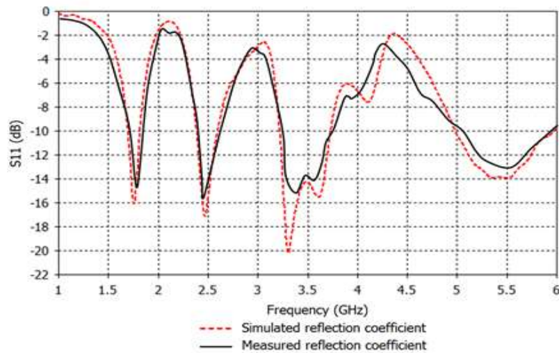
FIG. 3. The simulated and measured reflection coefficient of the proposed antenna.
