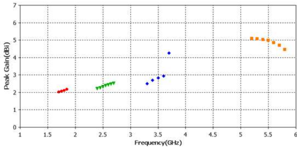
FIG. 6. Peak gain of the proposed antenna.
