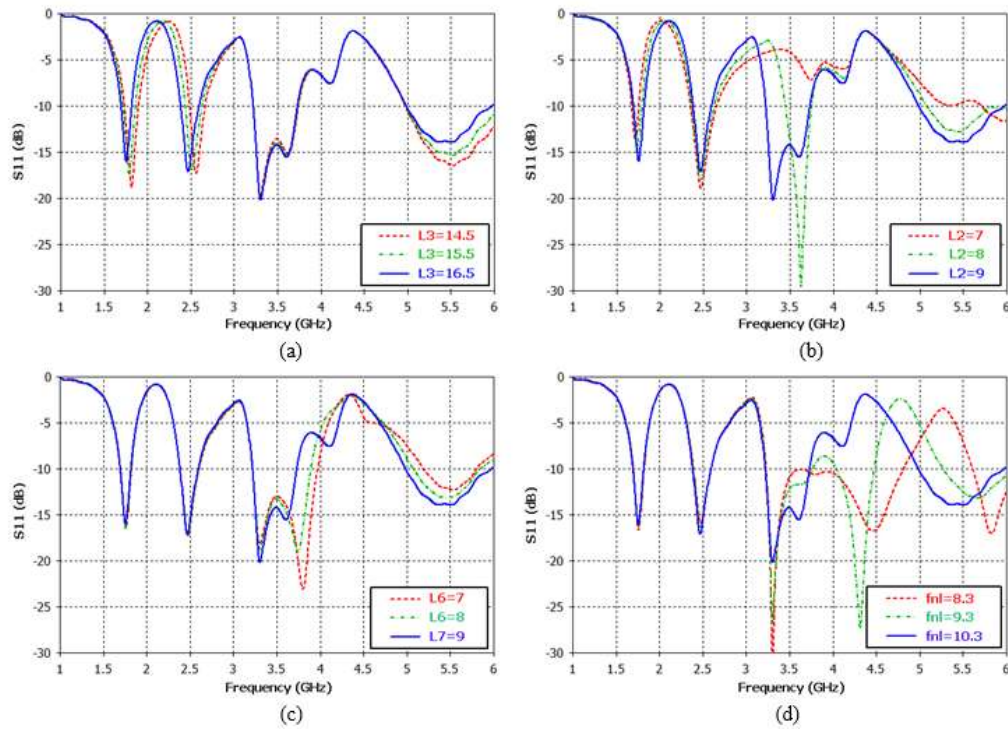
FIG. 2. The Simulated Reflection Coefficients of the Proposed Antenna with Different Values of L_3 , L_2 , L_6 , and f_{nl} (a) L_3 , (b) L_2 , (c) L_6 , (d) f_{nl}
