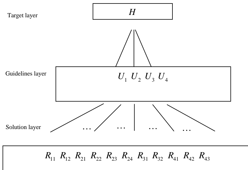
Figure 3: Hierarchical model
