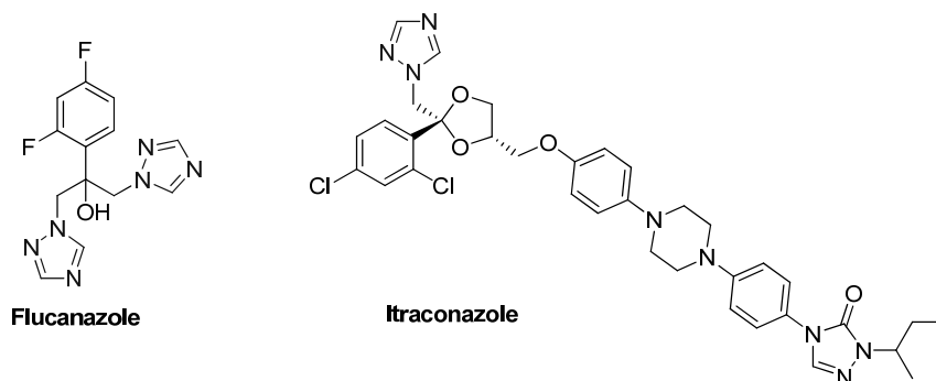
Fig. 2: Structures of flucanazole, itraconazole drugs containing 1, 2, 4 triazole core unit
