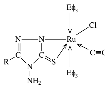
(R = \text{C}_6\text{H}_5\text{-}/\text{C}_6\text{H}_5\text{CH}_2 ; E = P/As) Oh-str. of [\text{RuCl}(\text{CO})(\text{E}\phi_3)_2\text{L}]
