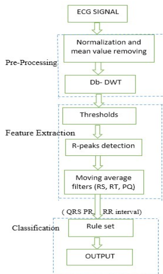
Fig. 1: Block diagram of algorithm
