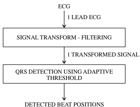
Fig. 2: Pan-Tompkins beat detection algorithm work flow
