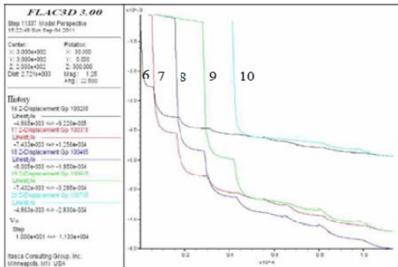
Figure 7 : Displacement change at No.6~10 monitoring points
