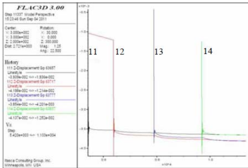
Figure 8 : Displacement change at No.11~14 monitoring points
