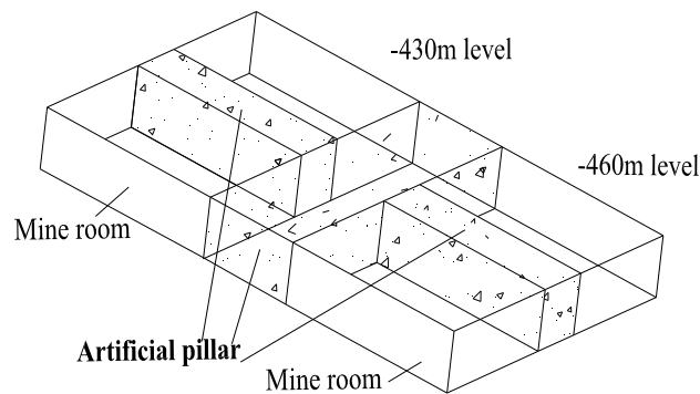
Figure 1 : Layouts of mine room and artificial pillar
