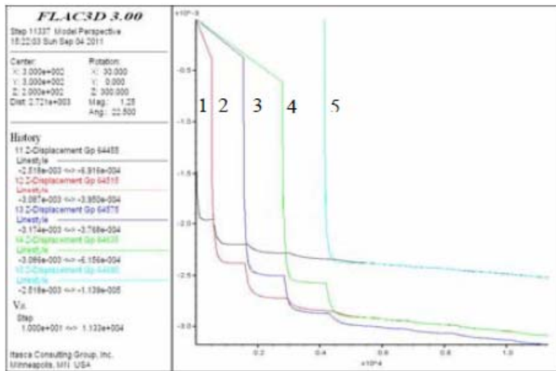
Figure 6 : Displacement change at No.1~5 monitoring points
