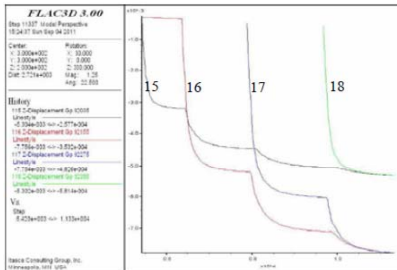
Figure 9 : Displacement change at No.15~18 monitoring points
