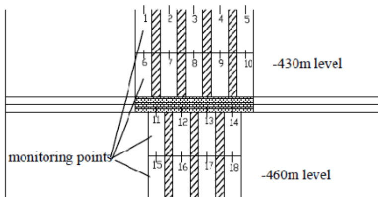
Figure 5 : Different stope structure displacement monitoring point arrangement plan
