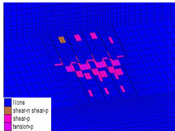
Figure 4 : Plastic zone distribution in pillars
