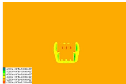
Figure 3 : Contour map of maximum principal stress
