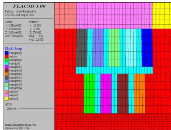
Figure 2 : Model of mine room and artificial pillar
