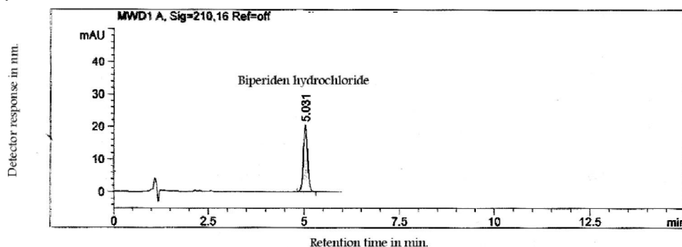
HPLC chromatogram of Achitnone® tablets containing 40 µg.mL -1 biperiden hydrochloride in methanol.
