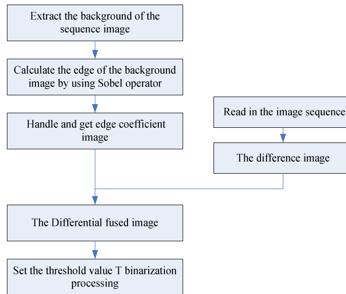
Figure 1 : The flow chart of adjacent frame difference based on the edge information
