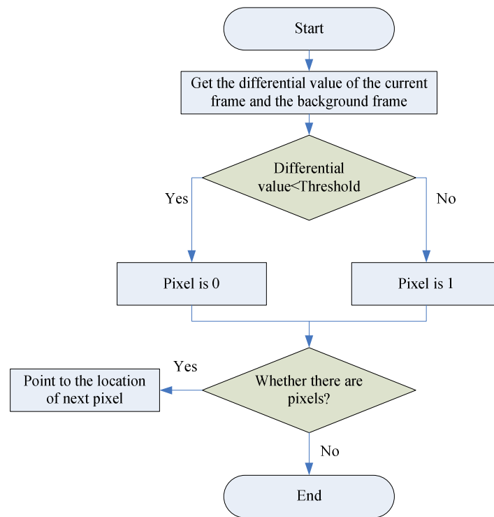
Figure 2 : The flowchart of background subtraction
