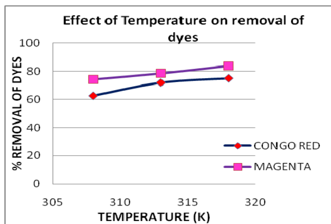
Fig. 2: Effect of temperature on removal of dyes
