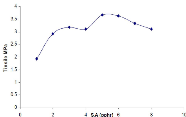
Figure 4 : Effect of (Satiric acid) on the SBR Tensile
