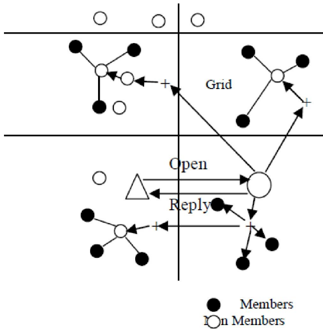
Figure 8 : Data delivery in hgmr [19]
