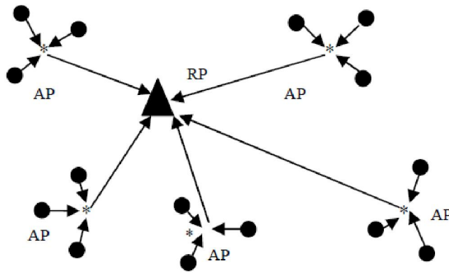
Figure 7 : Group management in hrpm [2]
