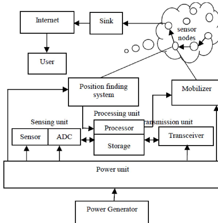
Figure 1 : Components of a sensor node 1
