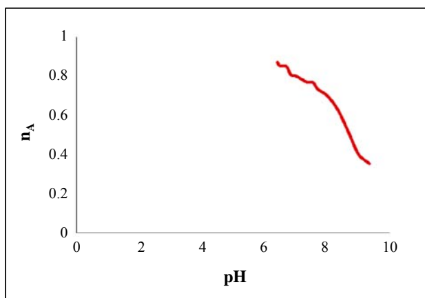
Fig. 5: Formation of n_A Vs pH ligand-L2
