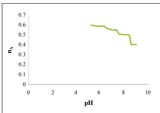
Fig. 6: Formation of n_A Vs pH ligand-L3
