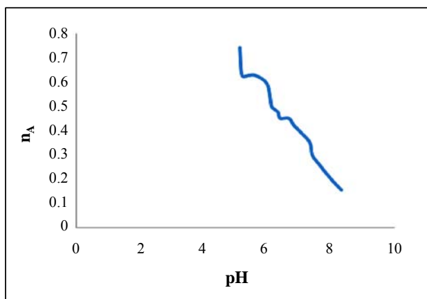
Fig. 4: Formation of n_A Vs pH ligand-L1
