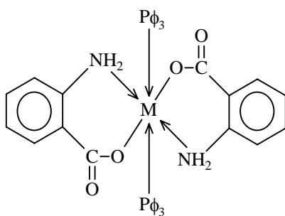
Octahedral Structure of [MA 2 (Pφ 3 ) 2 ]
