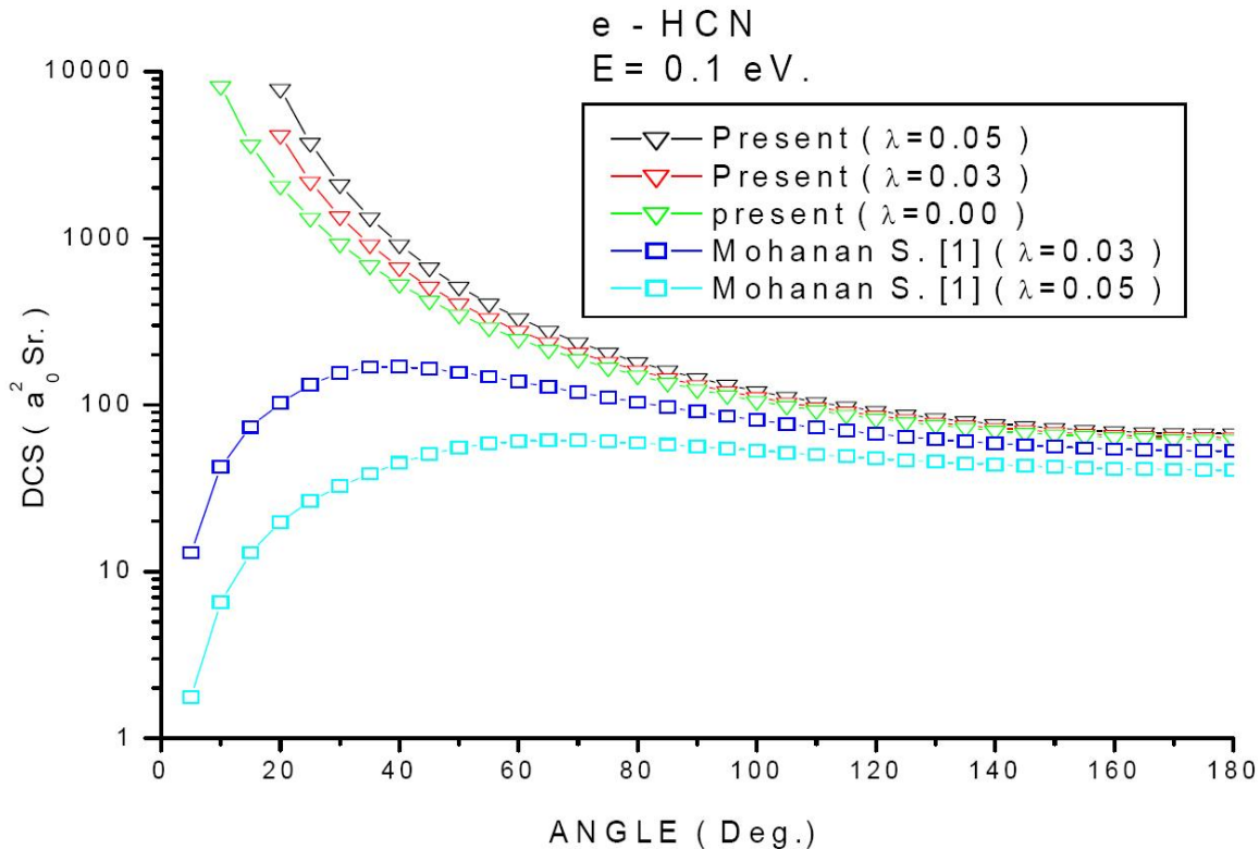
Figure 1 : Differential cross section of e-HCN at E=0.1 eV., Triangle line represents present data and square line gives the values from Mohanana S. [1]
