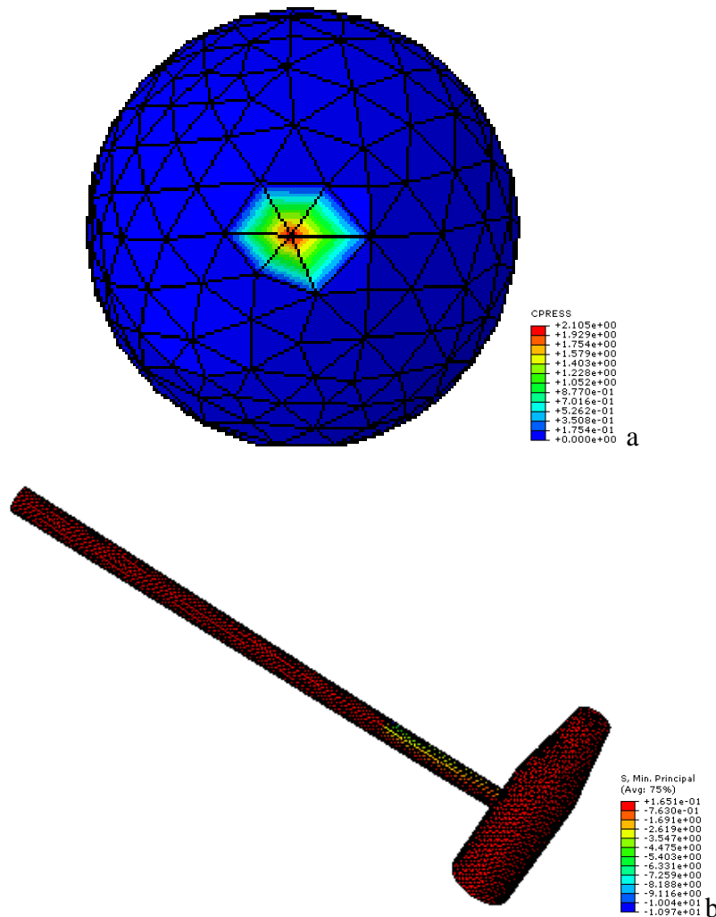
Figure 3 : The contact area at the ball during the collision process (a), and minimal stress of mallet (b)
