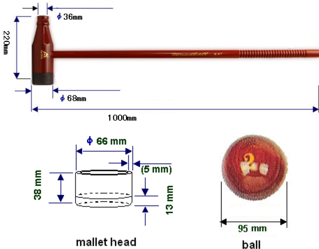
Figure 1 : The geometry information of woodball components
