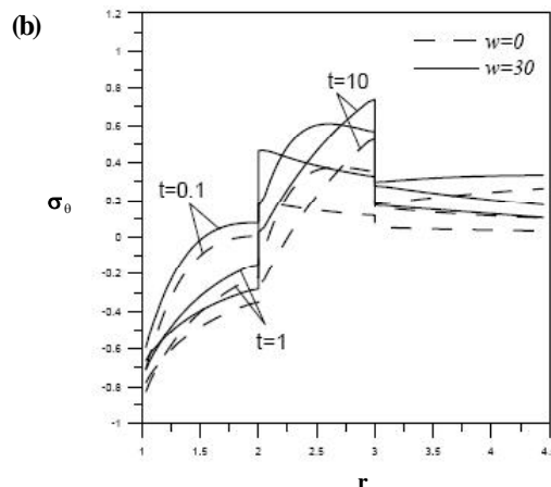
Figure 11 : Circumferential stress along radial direction and outer boundary being convection
