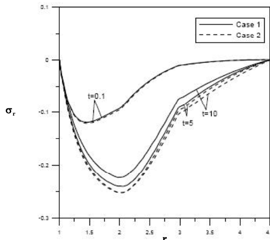
Figure 4 : Radial stress distribution along radial direction for angular velocity w=10
