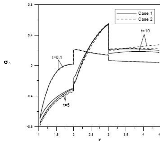
Figure 5 : Circumferential stress along radial direction for angular velocity w=10
