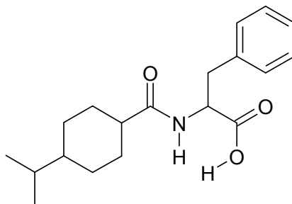
Nateglinide
