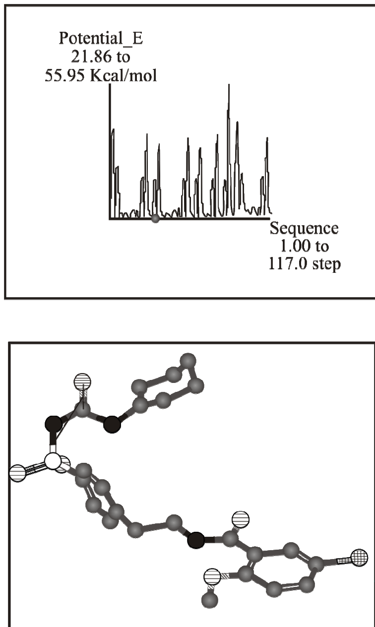
Fig. 5: Conformation analysis potential energy map and lowest energy state of glyburide
