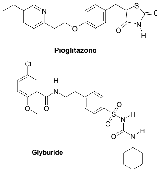
Fig. 1: Structures of molecules considered for analysis
