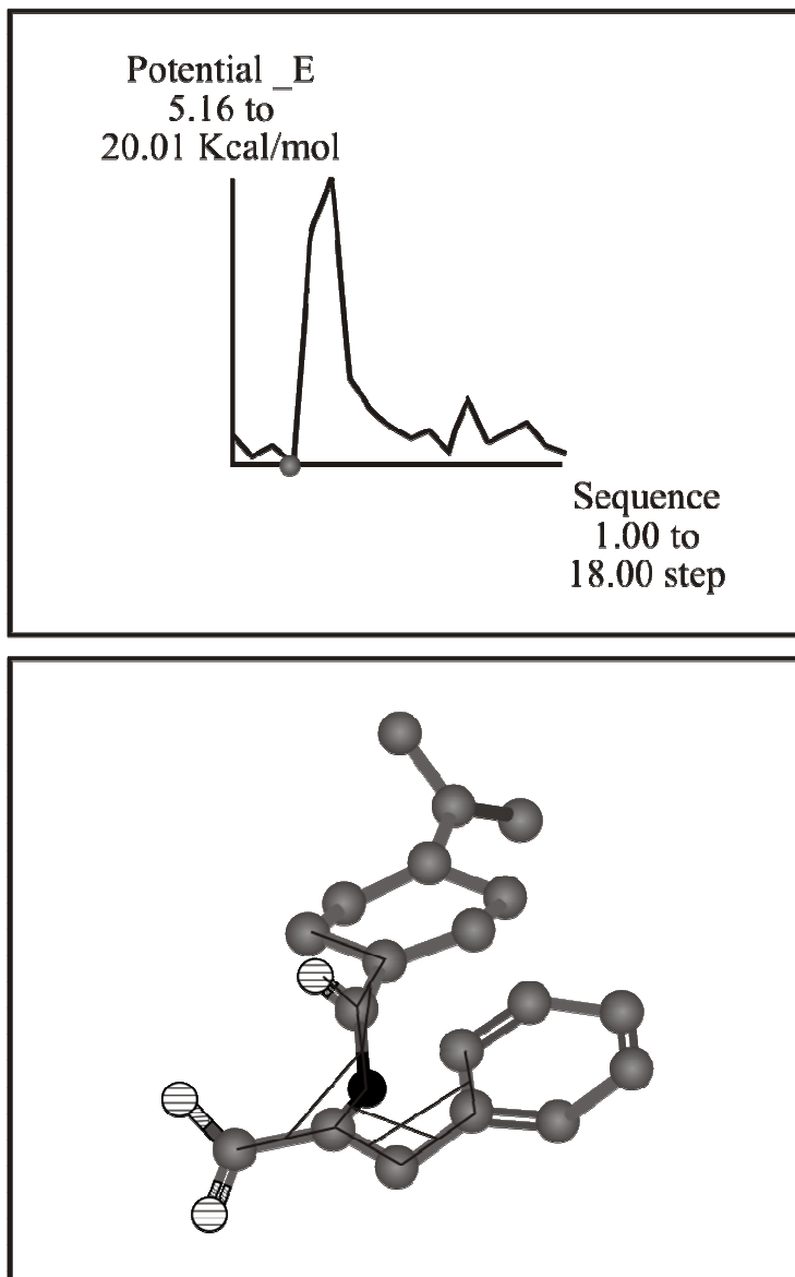
Fig. 2: Conformation analysis potential energy map and lowest energy state of nateglinide
