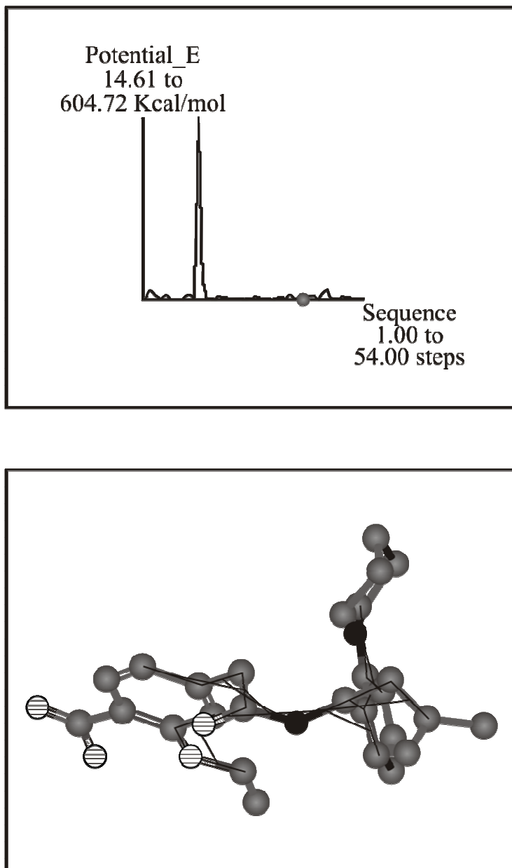
Fig. 4: Conformation analysis potential energy map and lowest energy state of repaglinide
