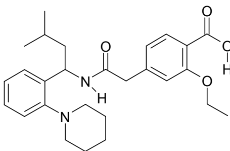
Repaglinide
