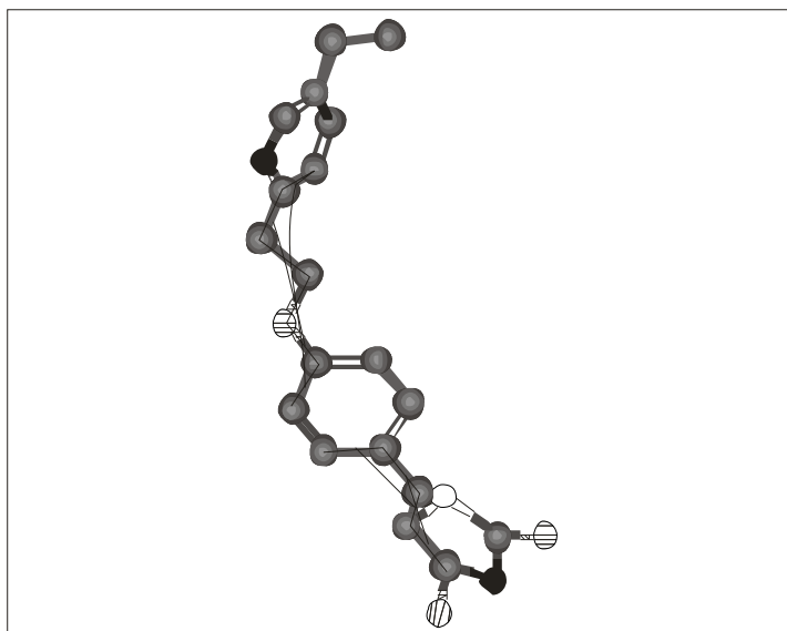
Fig. 3: Conformation analysis potential energy map and lowest energy state of pioglitazone
