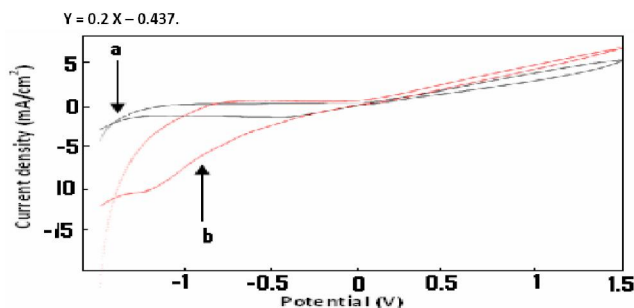
Figure 4 : CVs of eugenol polymer/GC modified electrode in pH 6.0, 0.1M \text{Na}_2\text{SO}_4 , [AA] = (a) 0 M, (b) 3mM, scan rate 100 mV/s.
