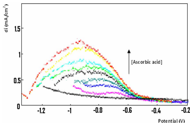
Figure 5 : Square voltammograms at eugenol polymer/GC modified electrode for different concentrations of ascorbic acid.
