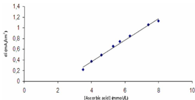
Figure 6 : Calibration curve for AA in \text{Na}_2\text{SO}_4 .
