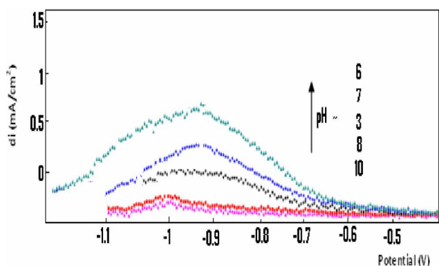
Figure 8 : Square wave voltammograms of 3 mMAA in 0.1 M \text{Na}_2\text{SO}_4 at different pH values.
