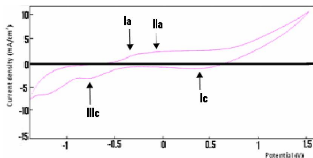
Figure 2 : Cyclic voltammograms of the eugenol film on GC electrode from the electrolyte 0.1 M KOH solution containing 4 mM eugenol monomers. Scan rate = 0.1 V/s, first cycle.
