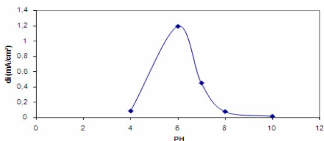
Figure 7 : Effect of pH on SWV peak of 3 mMAA in \text{Na}_2\text{SO}_4 0.1M.
