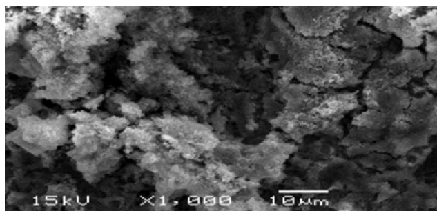
Figure 3 : SEM image of eugenol polymer film modified electrode.
