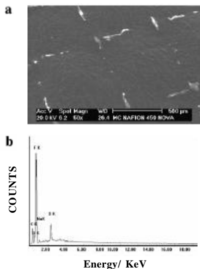
Figure 5: (a) New cation-exchange membrane (NAFION 450) micrograph and (b) respective EDS spectra
