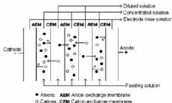
Figure 1: Electro dialysis technique principle
