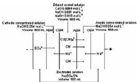
Figure 2: Five- compartment electro dialysis cell and the expected transport of the ionic species
