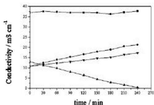
Figure 9: Behavior of the solution conductivity in the electro dialysis cell compartment during 240 minutes of electro dialysis with a 20\text{mA cm}^{-2} current density. (■) Electrodes (●) Anodic (▲) Central (▼) Cathodic
