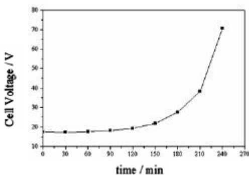
Figure 10: Behavior of the cell voltage during 240 minutes of electro dialysis with a 20\text{mA cm}^{-2} current density
