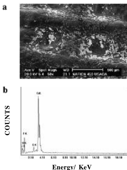
Figure 6: (a) Used cation-exchange membrane (NAFION 450) micrograph and (b) respective EDS spectra
