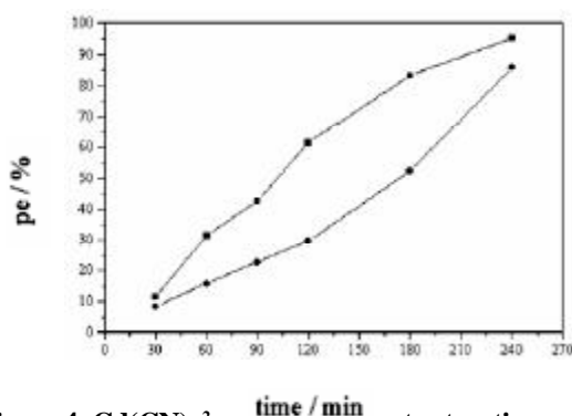
Figure 4: \text{Cd}(\text{CN})_4^{2-} and \text{CN}^- percent extraction as a function of the electro dialysis time with a 20 \text{ mA cm}^{-2} current density (●) \text{Cd}(\text{CN})_4^{2-} , \text{CN}^- (■)
