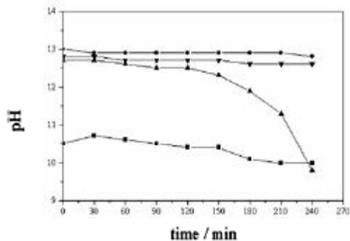
Figure 8: Behavior of the solution pH in the electro dialysis cell compartment during 240 minutes of electro dialysis with a 20\text{mA cm}^{-2} current density. (■) Electrodes (●) Anodic (▲) Central (▼) Cathodic
