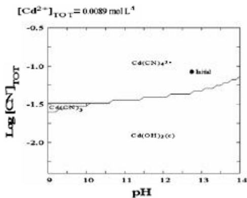
Figure 3: Speciation of cadmium and cyanide species as a function of the cyanide concentration and the solution pH ( 0.0089 \text{ mol L}^{-1} cadmium)
