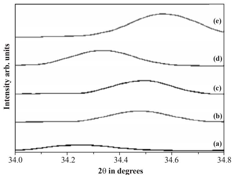
Fig. 2: Enlarged region of the (002) plane indicating the shift in XRD peaks due to the effect of number of dipping (a) 50, (b) 75, (c) 100, (d) 125 and (e) 150
