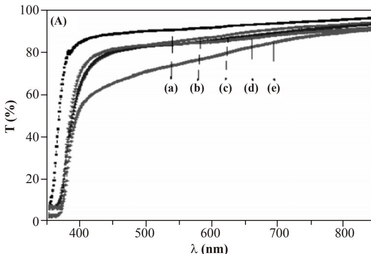
Fig. 4: Optical transmittance spectra of ZnO thin films prepared from different dipping (a) 50, (b) 75, (c) 100, (d) 125 and (e) 150
