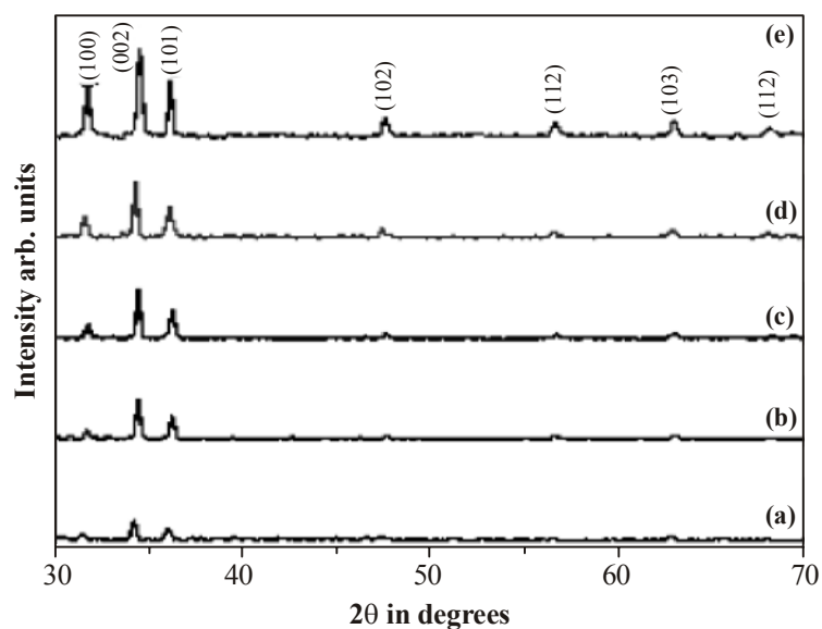
Fig. 1: The effect of number of dipping on the XRD patterns of ZnO thin films (a) 50 (b) 75 (c) 100 (d) 125 and (e) 150
