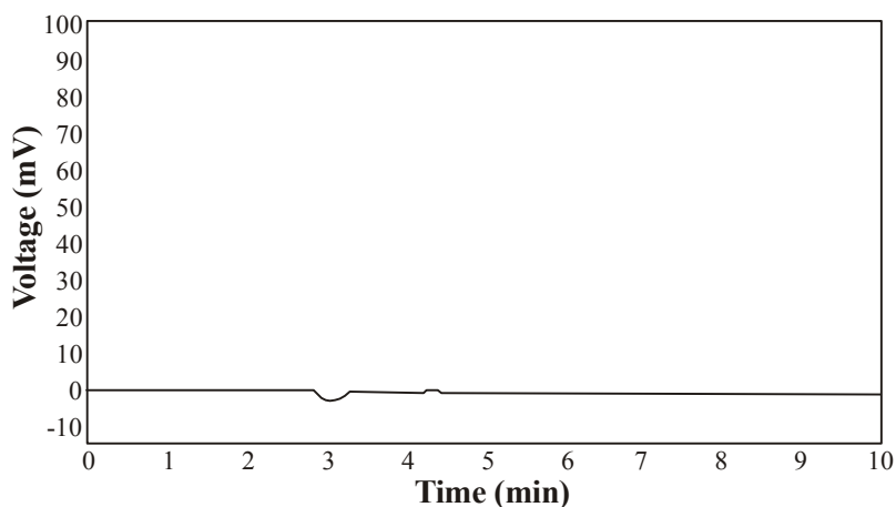
Fig. 4: Chromatogram of excipients of TD (30 \mu\text{g/mL} )
