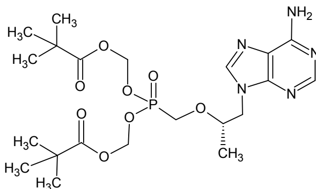
Fig. 1: Chemical structure of tenofovir disoproxil (TD)
