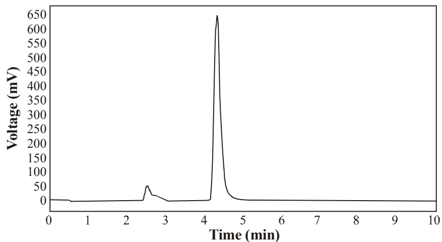
Fig. 2: Chromatogram of bulk drug TD (30 µg/mL). Retention time is 4.45 min
