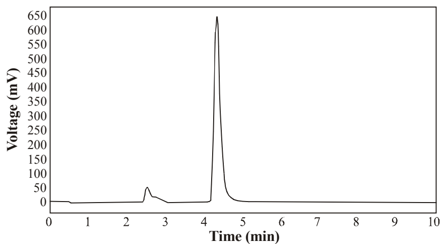
Fig. 3: Chromatogram of formulation TD (30 µg/mL). Retention time is 4.45 min
