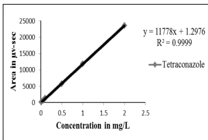
Fig. 7: Representative calibration curve of tetraconazole standard
