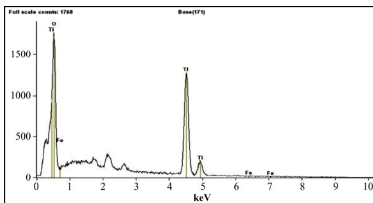
Fig. 1: EDX analysis of FeTiO 2 nanoparticles
