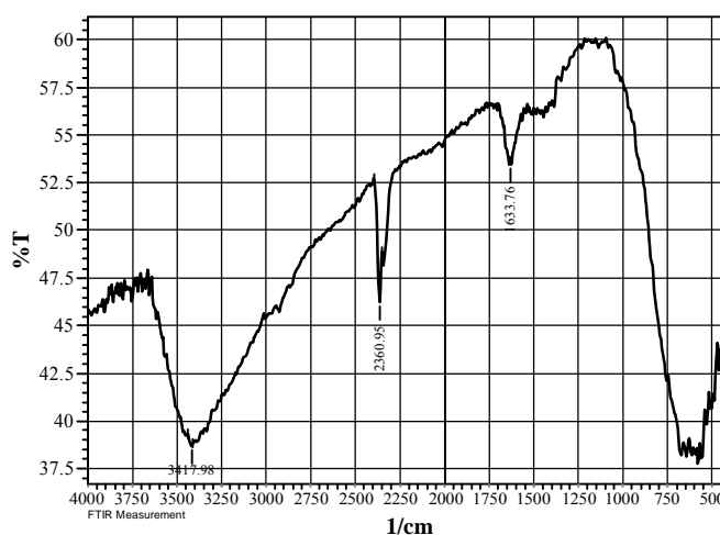
Fig. 3: FT-IR Spectra of FeTiO 2 nanoparticles
