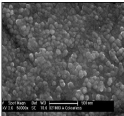
Fig. 2: SEM Image of FeTiO 2 nanoparticles
