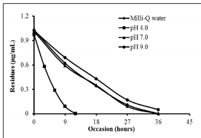
Fig. 8: Graph representing the dissipation curve of photocatalytic decontamination of tetraconazole in water under direct sunlight
