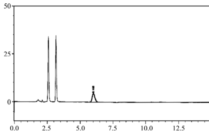
Fig. 4: Representative chromatogram of tetraconazole test item in acidic water- 3 rd hr
