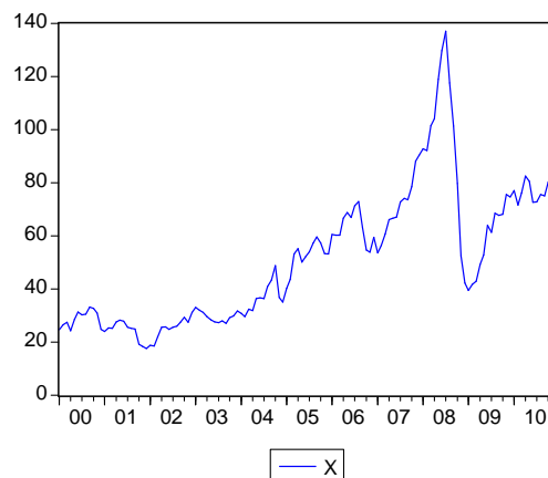
Figure 1 : The series of daqing crude oil price
