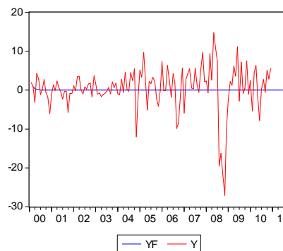
Figure 5 : The result of dynamic forecasting mode
