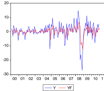
Figure 7 Fitting static renderings
