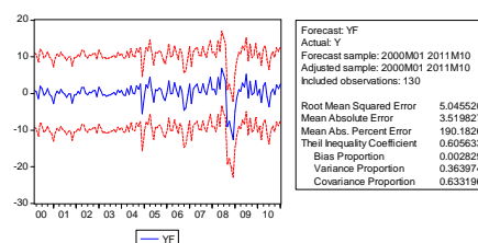
Figure 6 : Static forecasting mode
