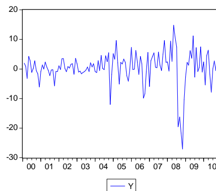
Figure 2 : Line charts of the first difference sequence
