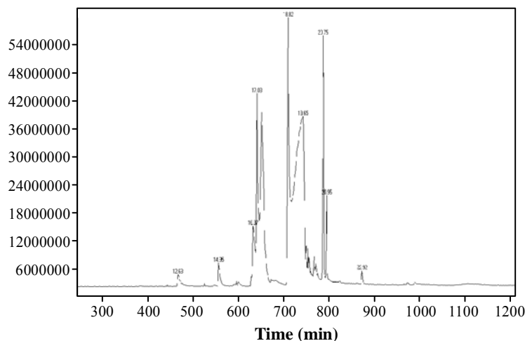
Fig. 1: GC/MS spectrum of Canola seed biodiesel
