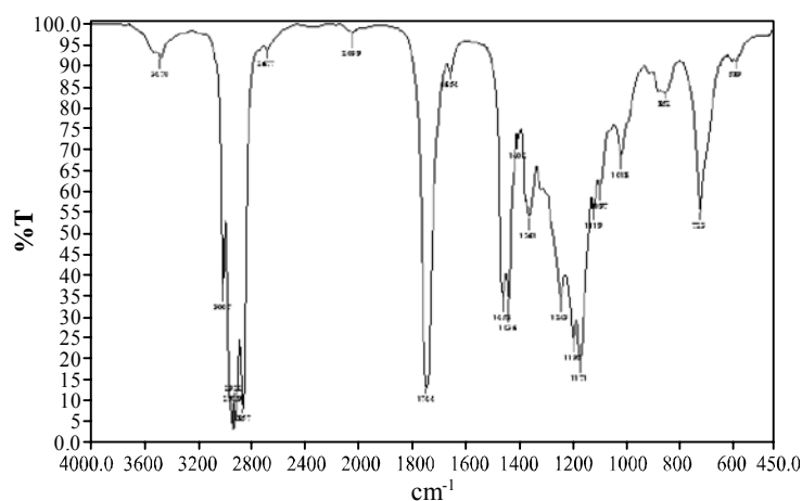
Fig. 2: FT IR spectrum of Canola seed biodiesel
