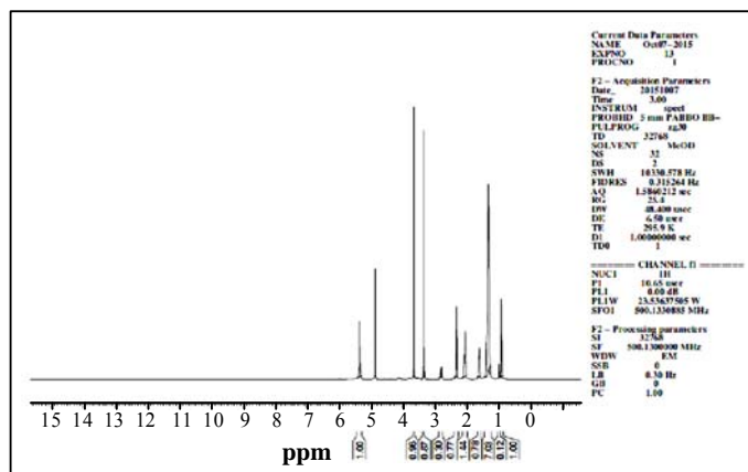
Fig. 3: 1 H NMR spectrum of Canola seed biodiesel
