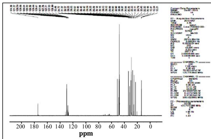
Fig. 4: 13 C NMR spectrum of Canola seed biodiesel
