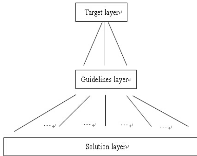
Figure 2 : Hierarchical model
